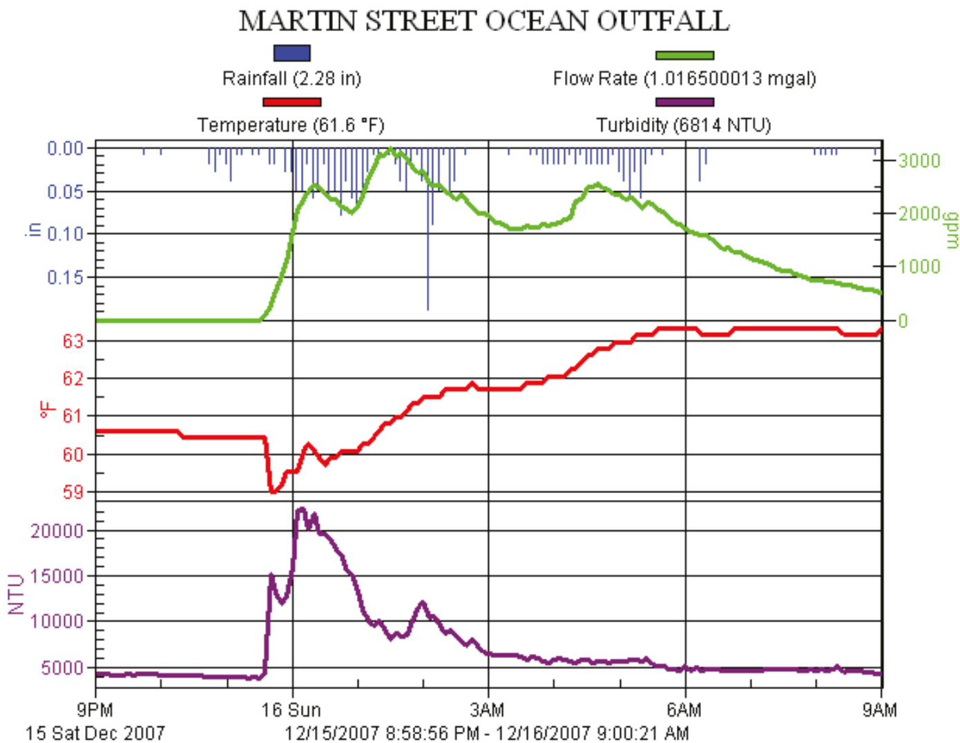
Figure 3. Patterns of rainfall, stormwater flow, water temperature, and turbidity throughout a winter rain storm.
